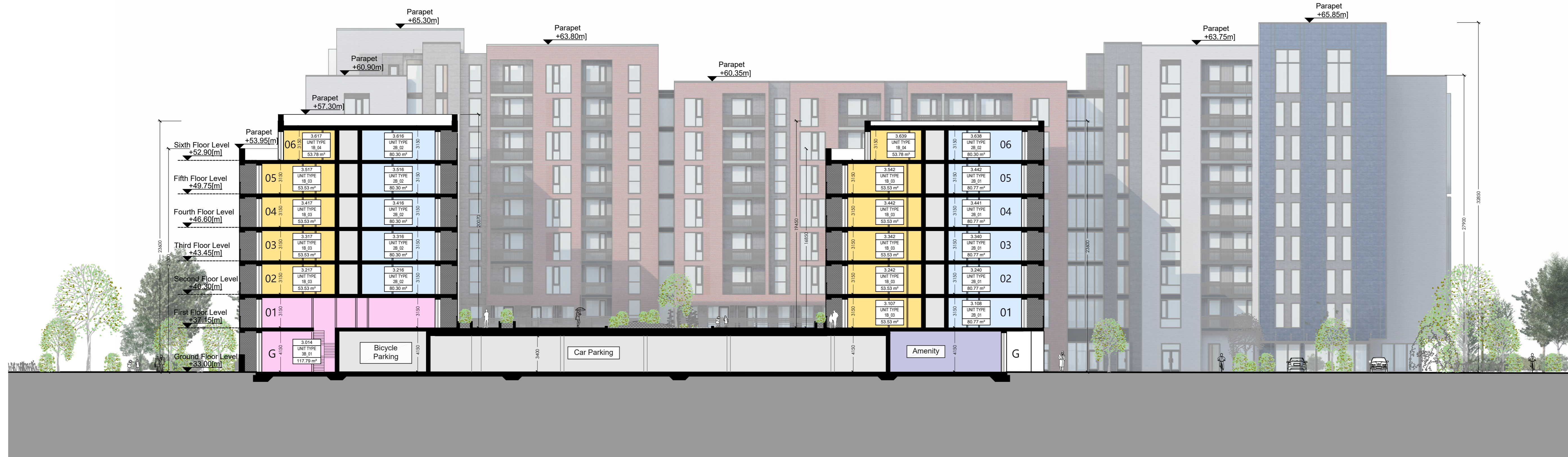
Section AA - Block 3 Scale 1:200 @A0
